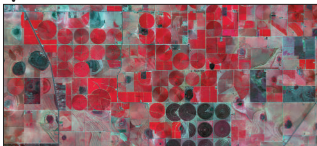
Irrigation satellite imagery (courtesy Texas Natural Resources Information Service/Texas Water Development Board).
